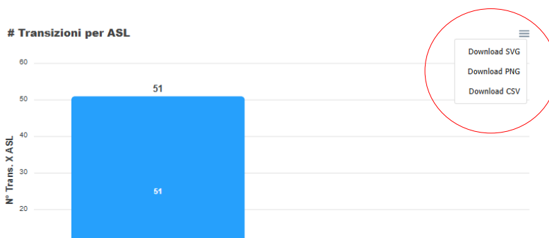
Figura 163 - Download File
