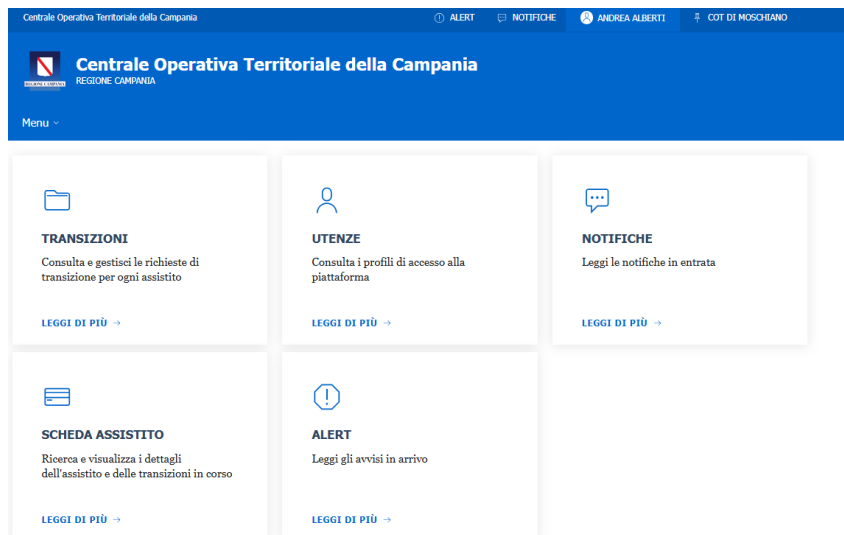
Figura 48 - Home Page
