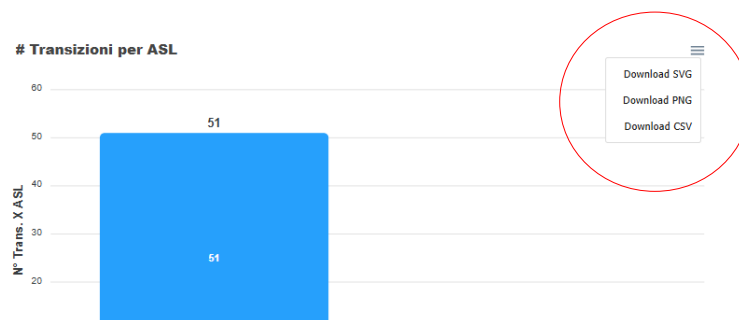
Figura 171 - Download File
