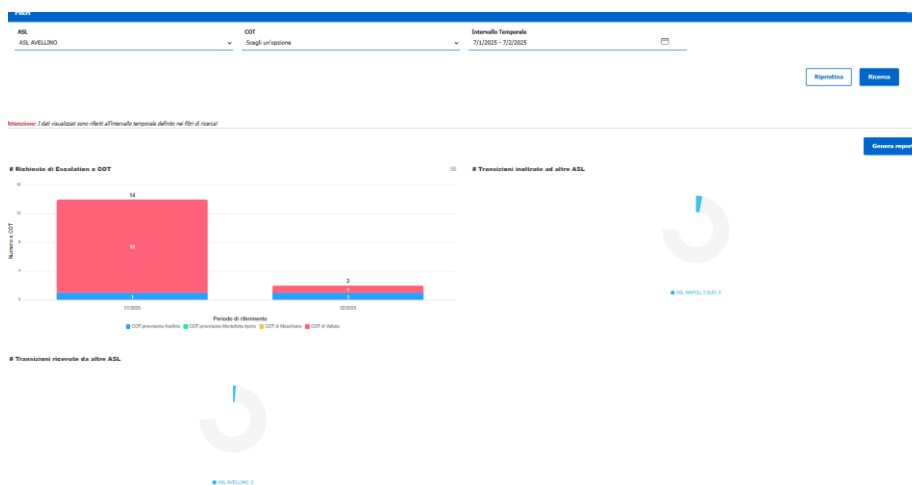
Figura 178 - Report Escalation
