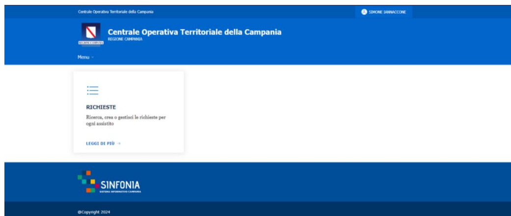
Figura 28 - Home Page
