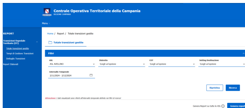
Figura 159 - Report
