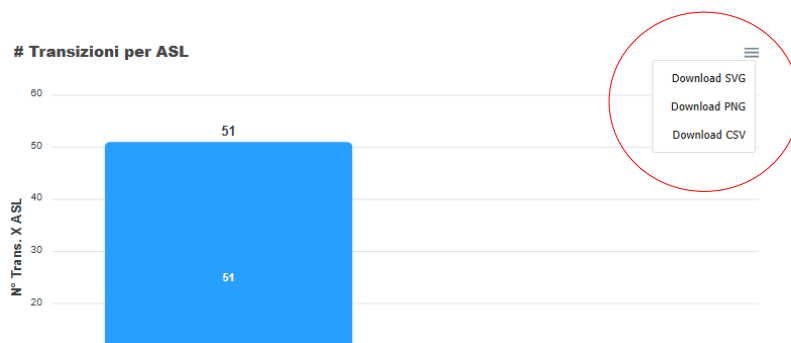
Figura 167 - Download File
