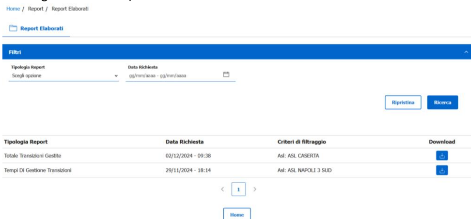
Figura 173 - Report Elaborati
